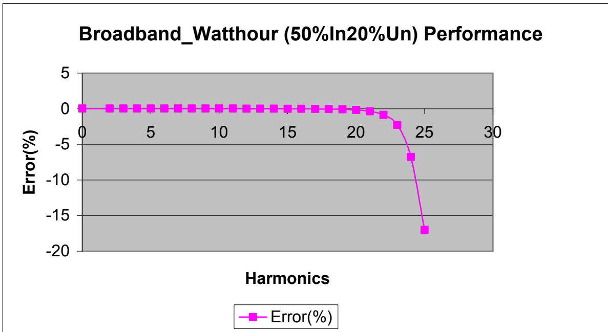
Figure 9: Broadband Watt-Hour Harmonic Performance
